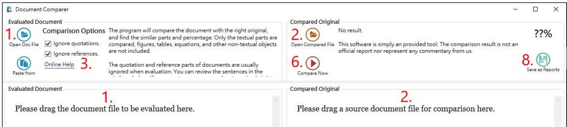
Fig 2. The main window
